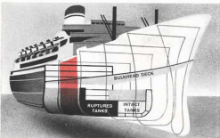
WHY DORIA SANK is indicated in drawing. Blow struck in red area, cutting from below waterline to main deck, destroying watertight integrity of bulkhead deck. Starboard fuel tanks (black), nearly empty at end of run, flooded, causing list. List automatically increased as more water poured in above bulkhead deck.
